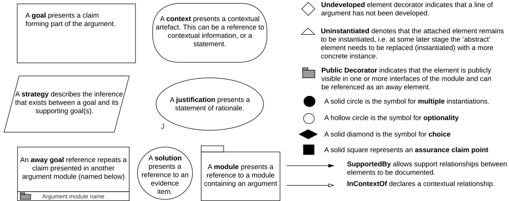
Fig. 2. Symbols and elements of a GSN argument. Extracted and adapted from Assurance Case Working Group [65]
